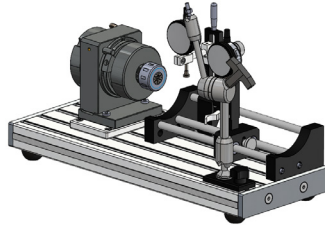
Beating measuring equipment
